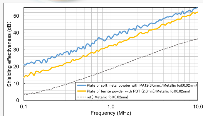
【Frequency response of magnetic shielding effectiveness】
