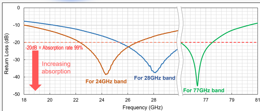
[Absorption properties of millimeter-wave absorbent sheets]
